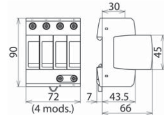
Dimension drawing DG M TT CI 275
