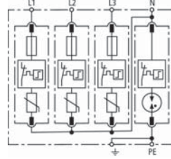
Basic circuit diagram DG M TT CI 275
